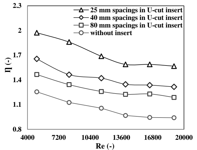
Fig.7: Variation of heat transfer enhancement efficiency with Reynolds number.
