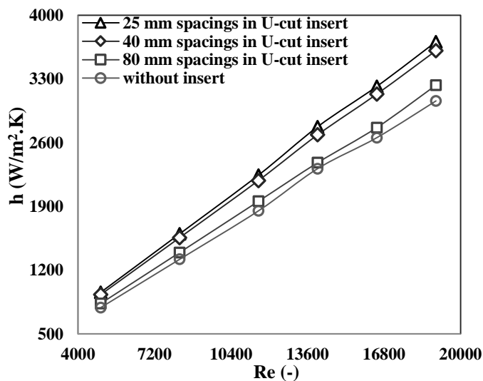
Fig.6: Variation of convective heat transfer coefficient with Reynolds number.
