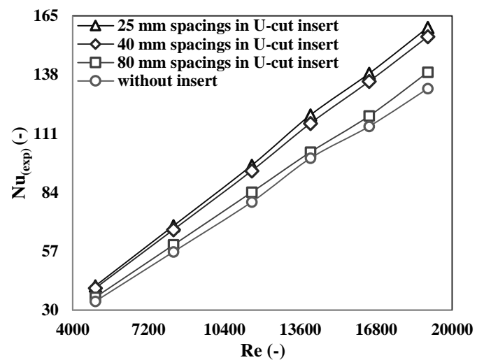
Fig.3: Variation of Nusselt number with Reynolds number.
