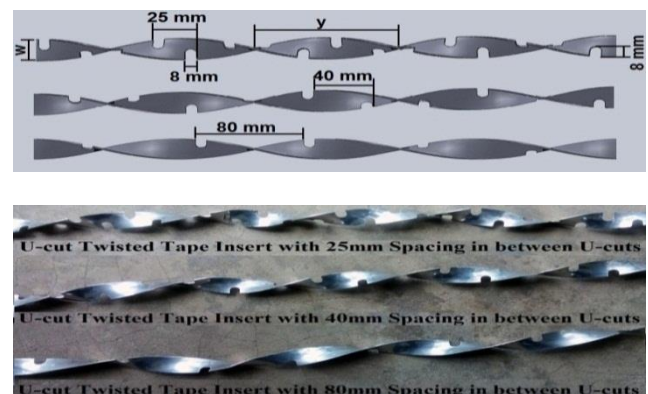
Fig.1: U-shape twisted tape inserts.
