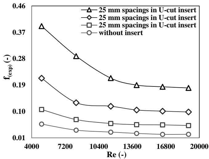
Fig.5: Variation of friction factor with Reynolds number.
